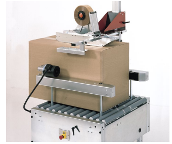
Raised side drives for high cases.
